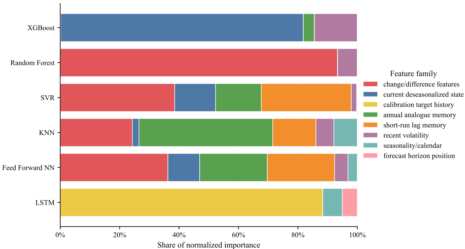
Model Reliance by Feature Family
